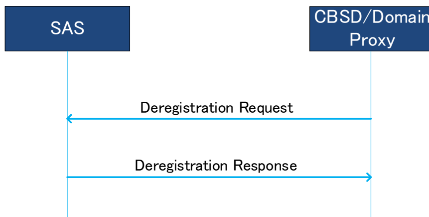
Figure 9: CBSD Deregistration Procedure.
