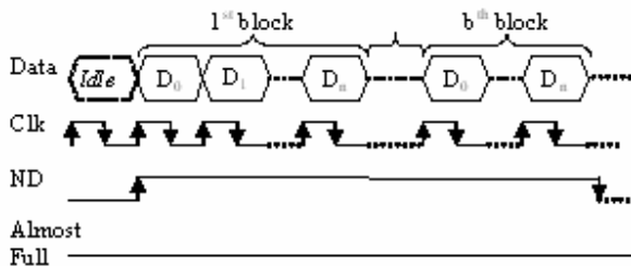
Figure 4. Data written by the GPIF, normal operation
