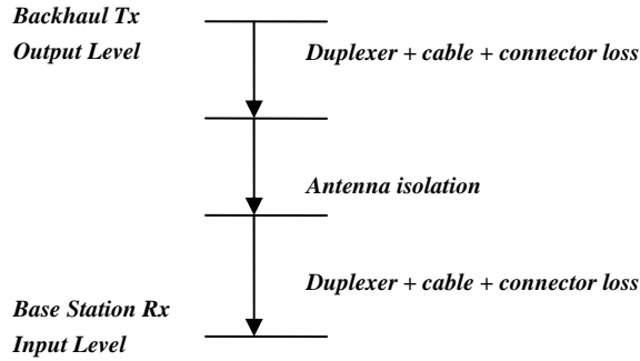
Figure 5: Calculation of required filtering and antenna isolation. It is assumed here that filtering is provided by the backhaul duplexer
